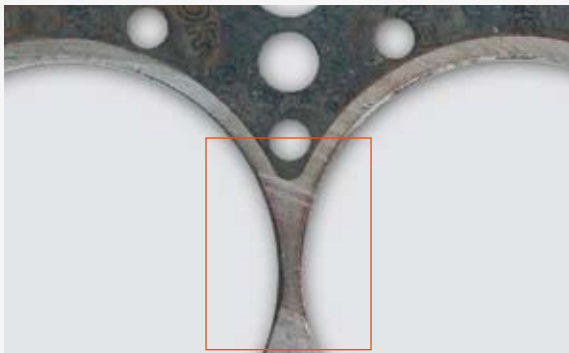
▲ Roughness of engine block and cylinder head surfaces leads to gas blowby between the combustion chambers.
