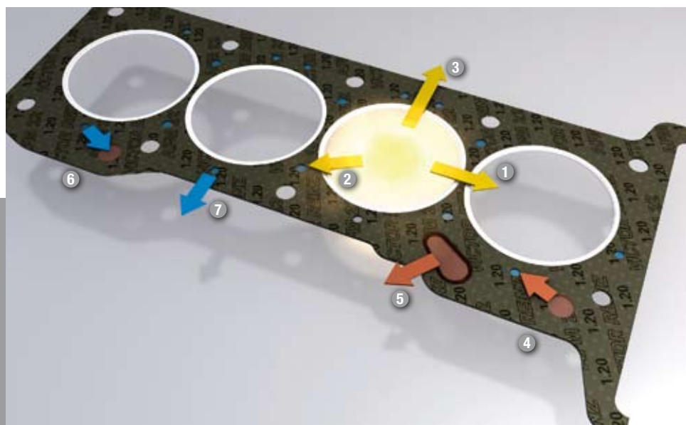
◀ Typical media leakages with composite cylinder head gaskets.
